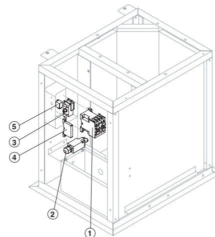
ELECTRIC PARTS
