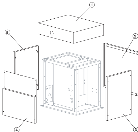
SHELL ASSY
