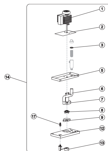
PUMP
