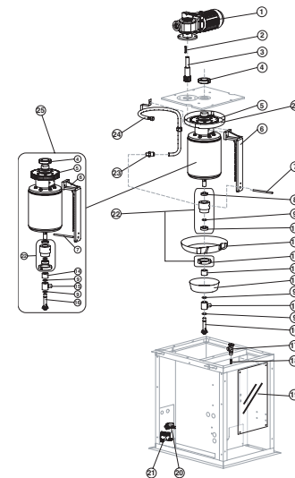
ELECTRIC PARTS
